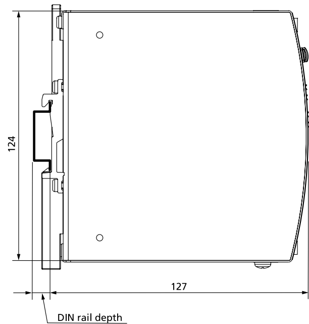
Fig. 22-2: Side view
