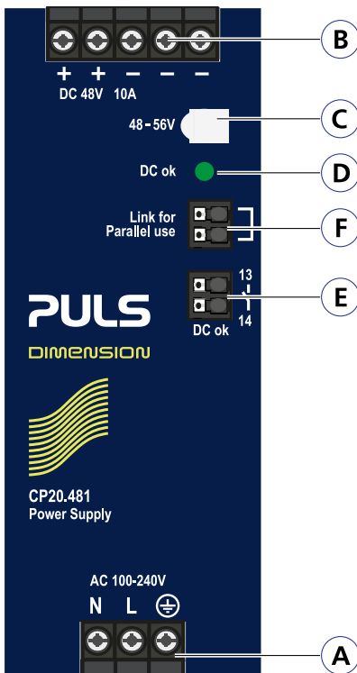
Fig. 14-1: Front side
