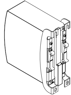
Fig. 23-3: Isometric view
