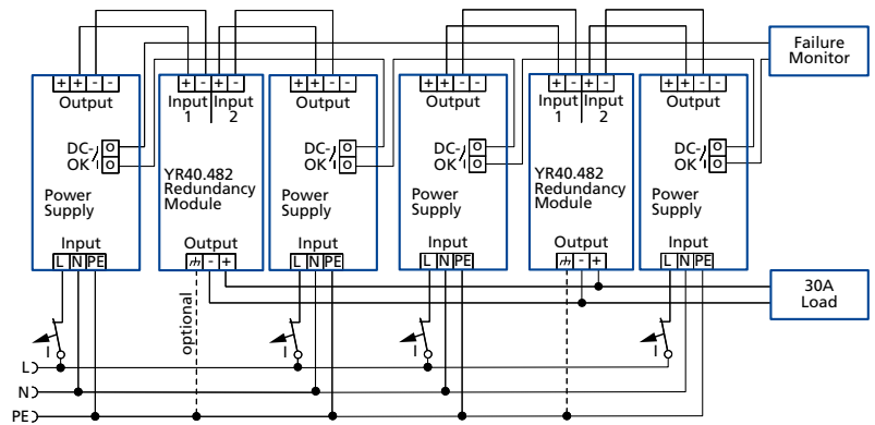
Fig. 24-6: N+1 Redundant configuration for 30A load current with multiple devices and redundancy modules
